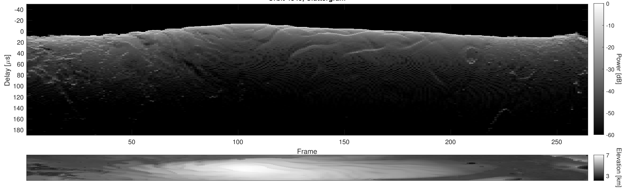
Orbit 4349, Cluttergram
