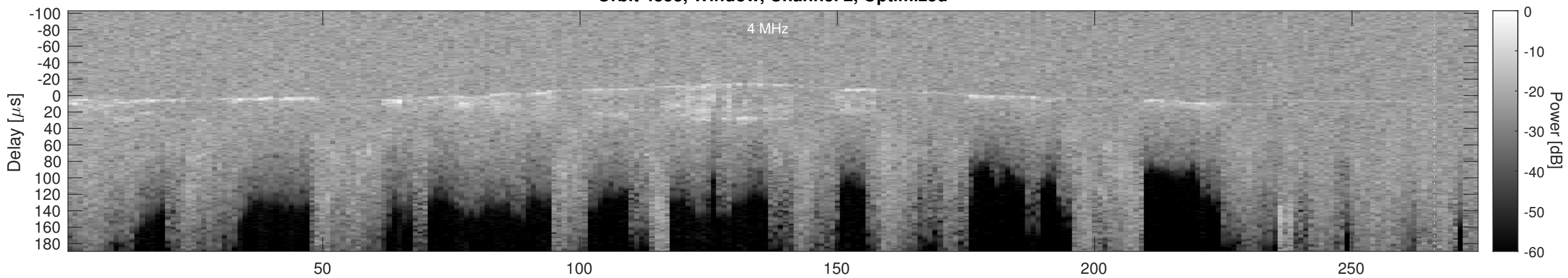
Orbit 4353, Cluttergram
