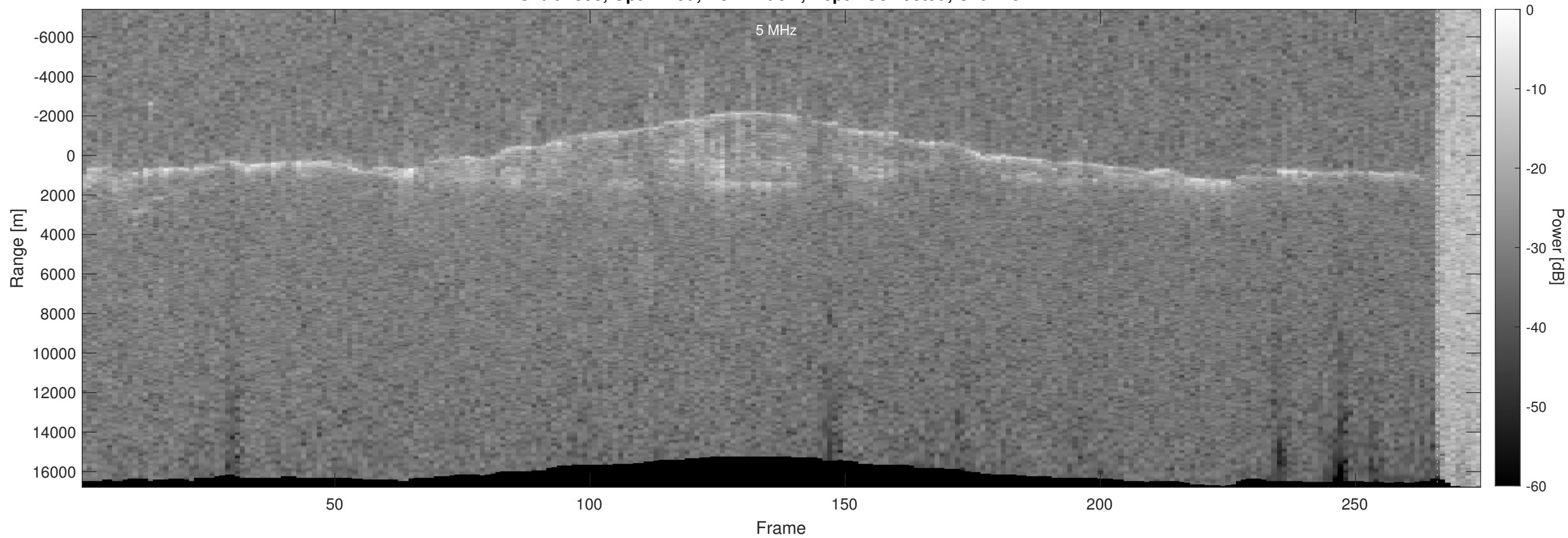
Orbit 4353, Optimized, No Window, Depth-Corrected, Channel 2
