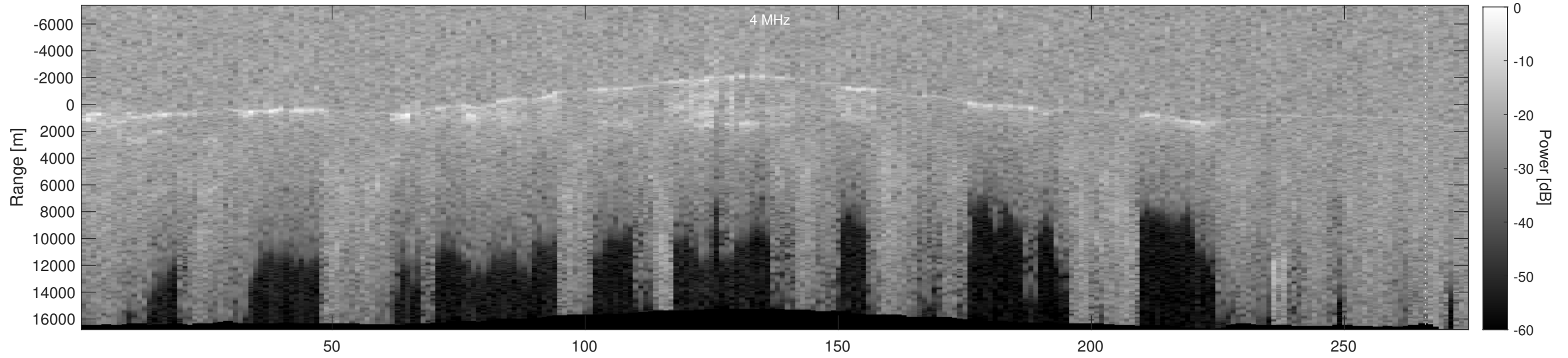
Orbit 4353, Depth-Corrected Cluttergram
