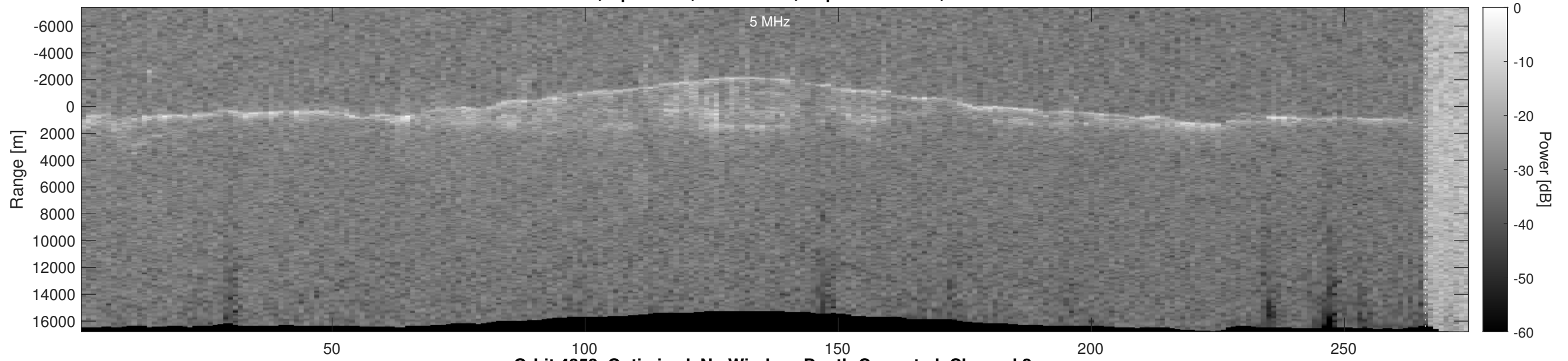
Orbit 4353, Optimized, No Window, Depth-Corrected, Channel 2
