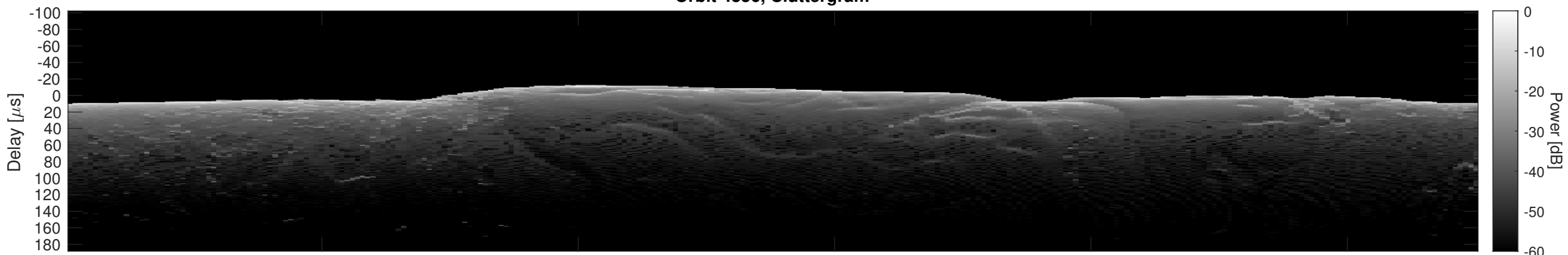
Orbit 4356, Cluttergram
