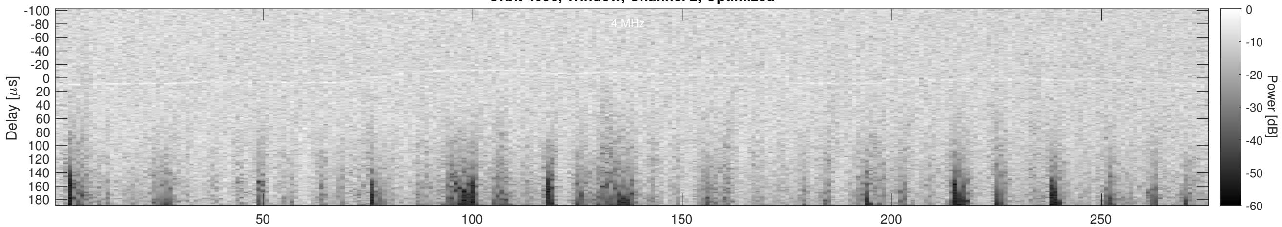
Orbit 4356, Cluttergram
