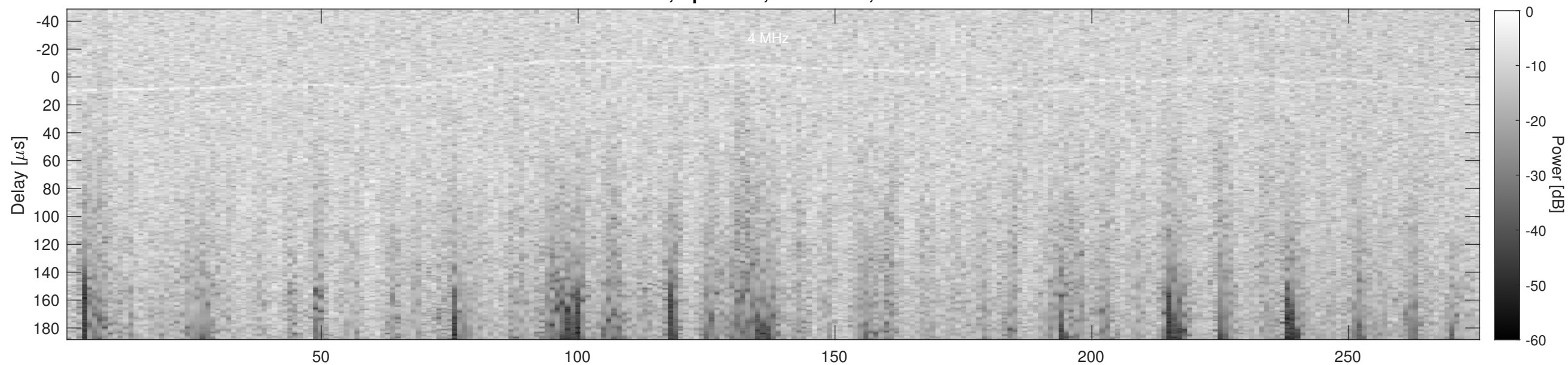
Orbit 4356, Cluttergram
