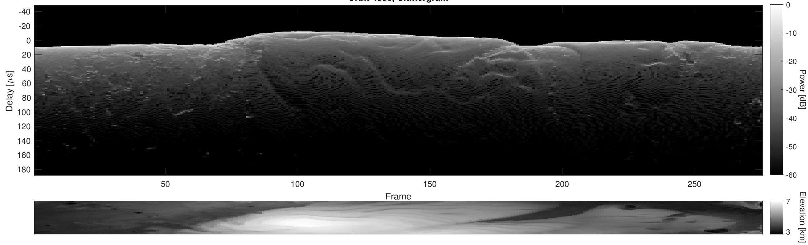
Orbit 4356, Cluttergram
