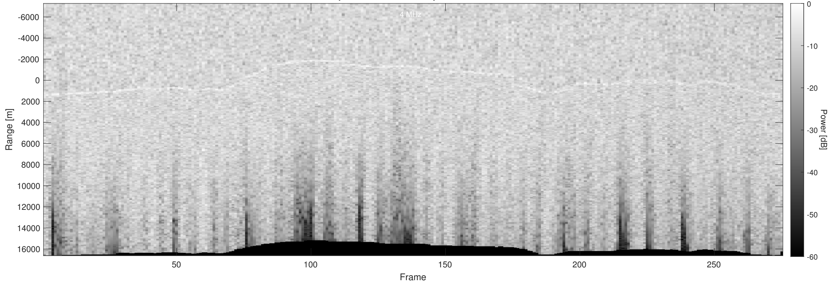
Orbit 4356, Optimized, Window, Depth-Corrected, Channel 2
