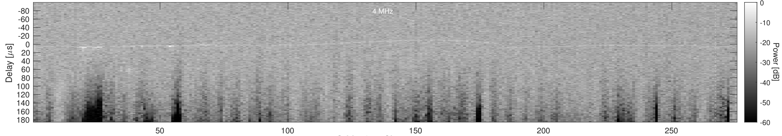
Orbit 4357, Cluttergram
