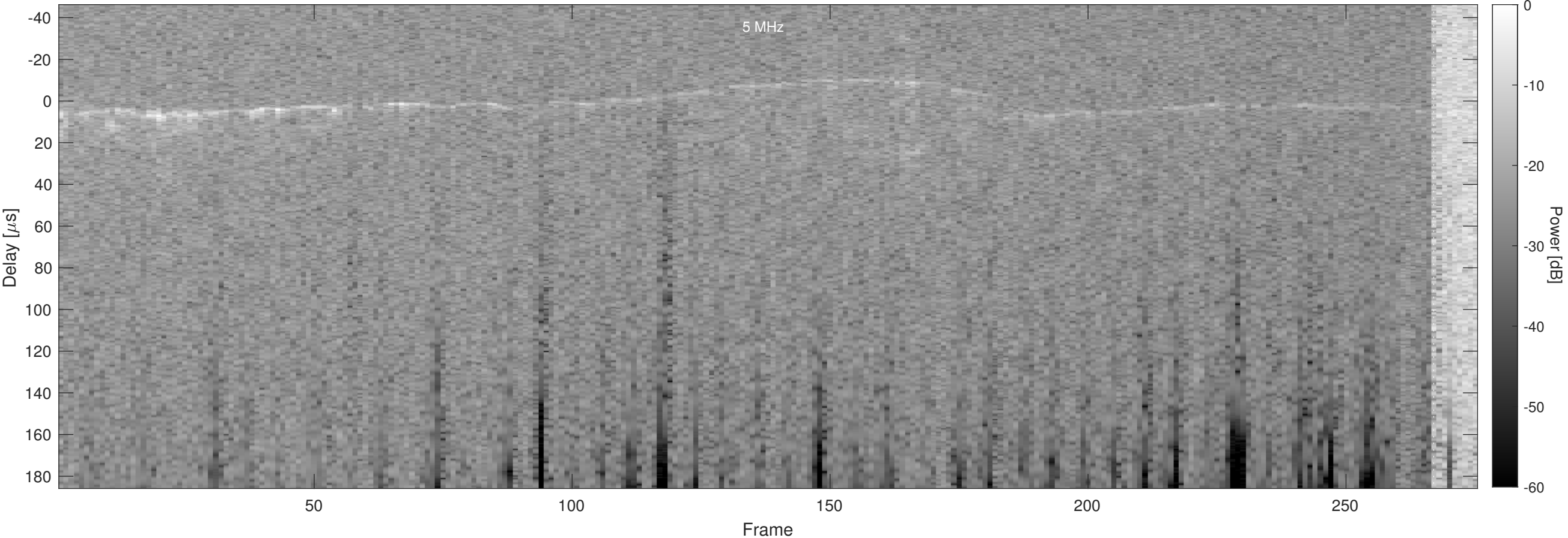
Orbit 4357, Optimized, No Window, Channel 2
