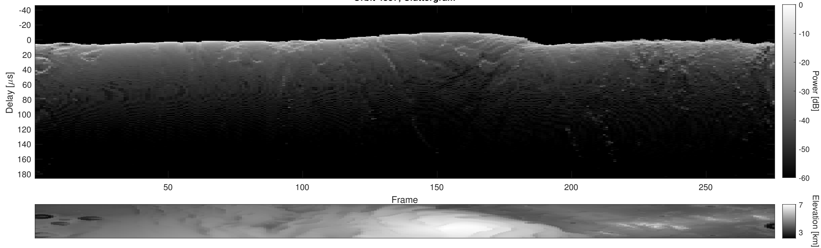
Orbit 4357, Cluttergram
