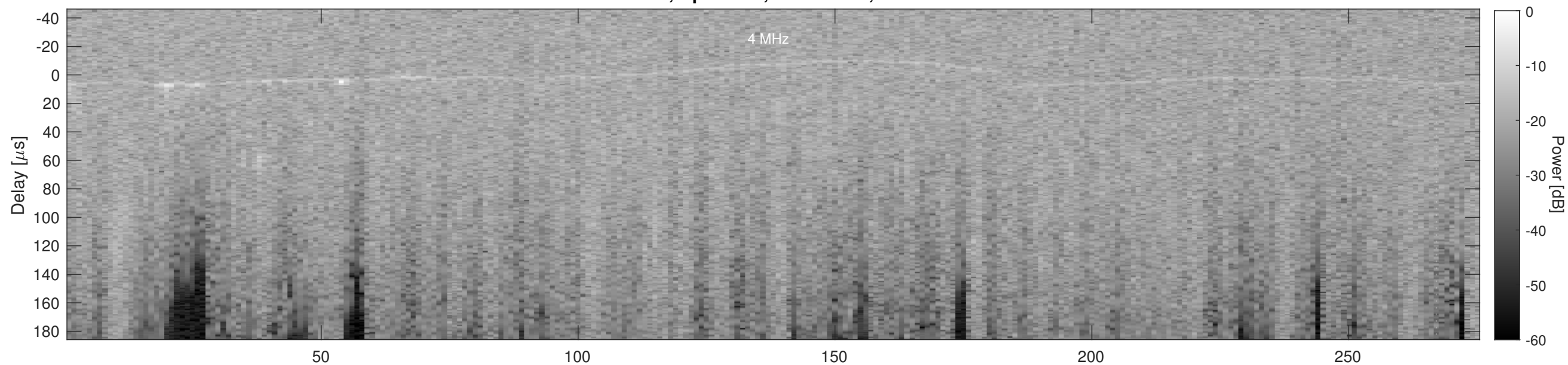
Orbit 4357, Cluttergram
