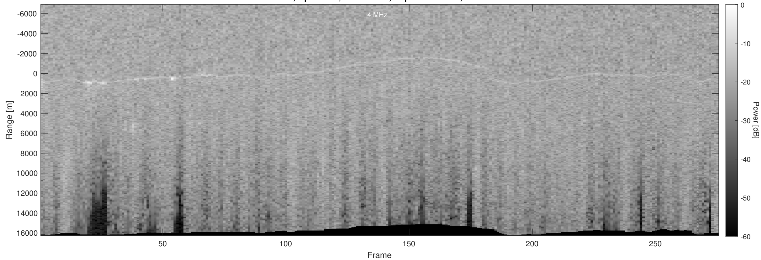
Orbit 4357, Optimized, No Window, Depth-Corrected, Channel 2
