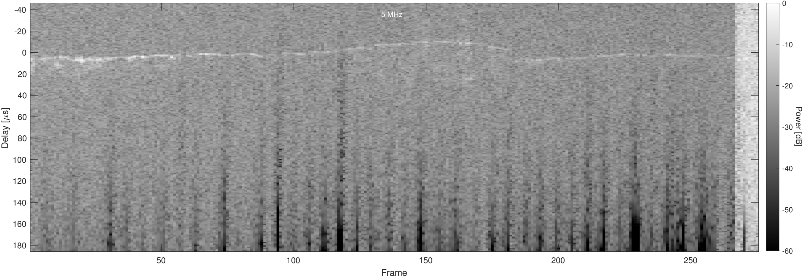
Orbit 4357, Optimized, Window, Channel 2
