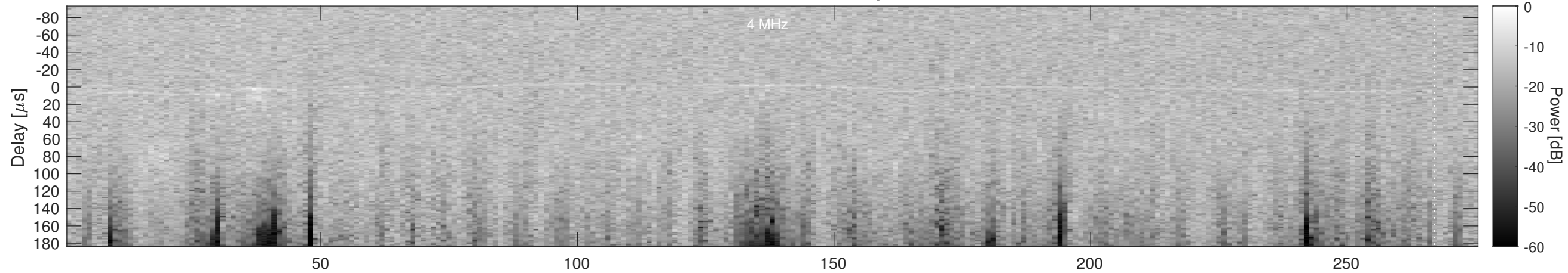
Orbit 4358, Cluttergram
