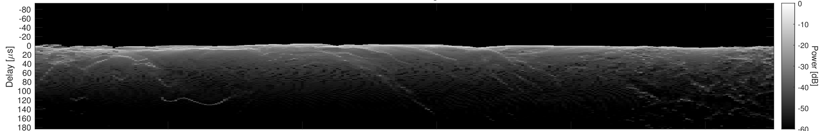
Orbit 4358, Cluttergram
