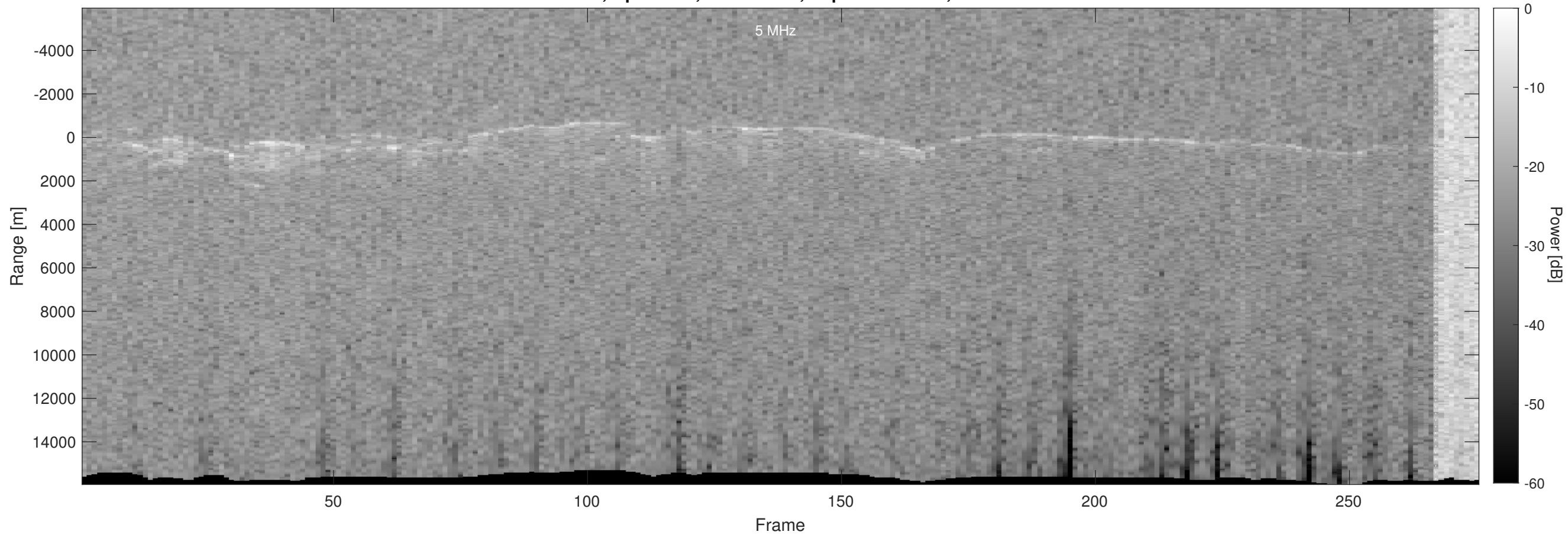
Orbit 4358, Optimized, No Window, Depth-Corrected, Channel 2
