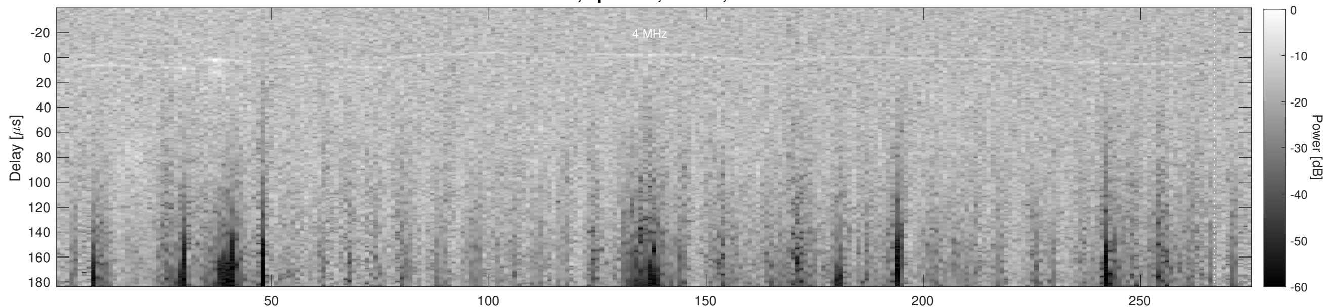
Orbit 4358, Cluttergram
