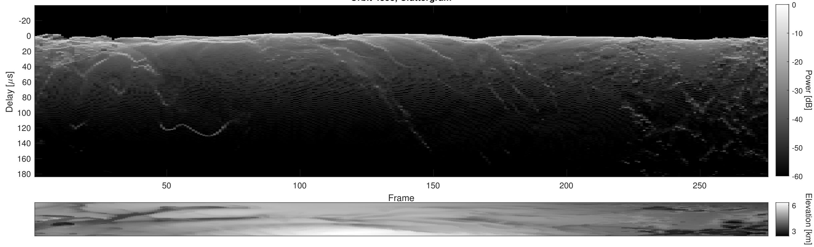
Orbit 4358, Cluttergram
