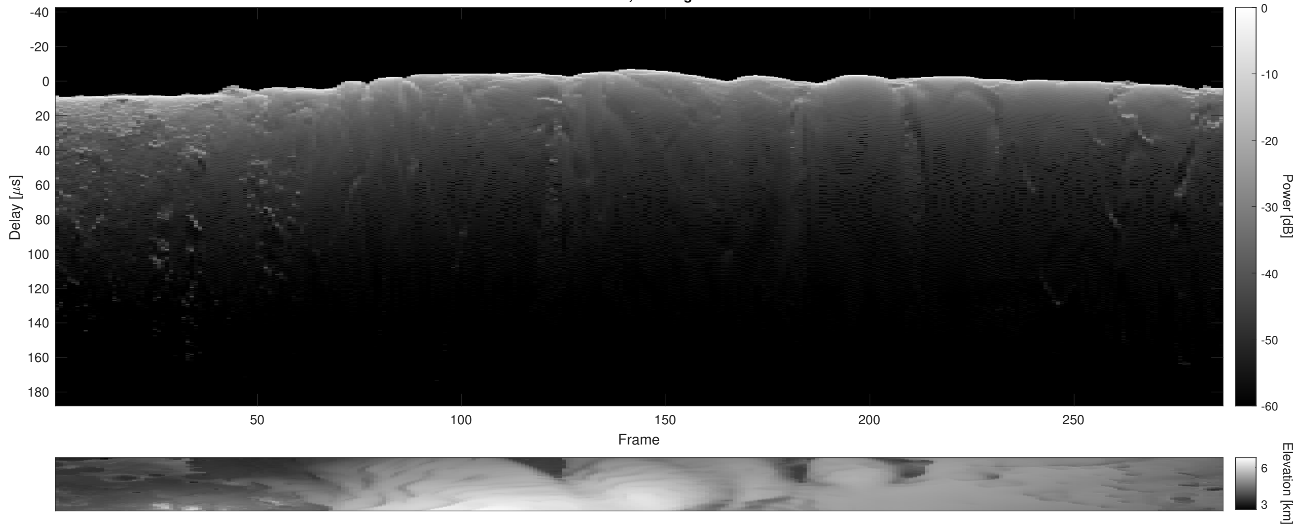
Orbit 4359, Cluttergram
