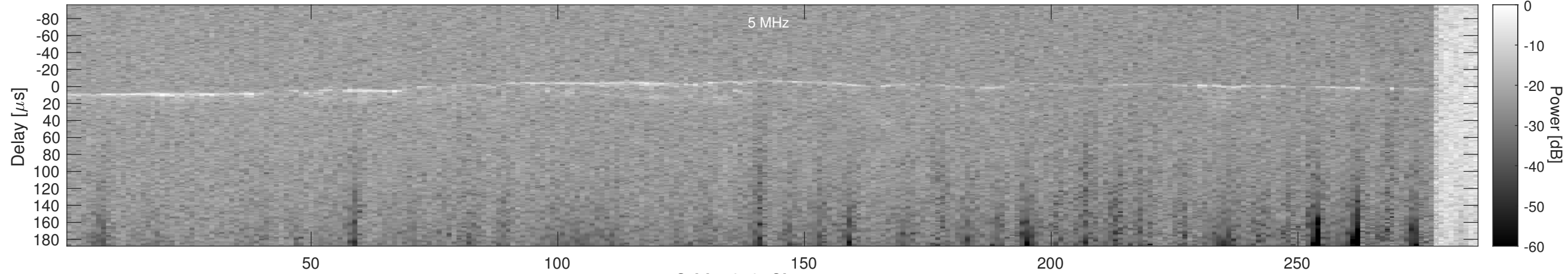
Orbit 4359, Cluttergram
