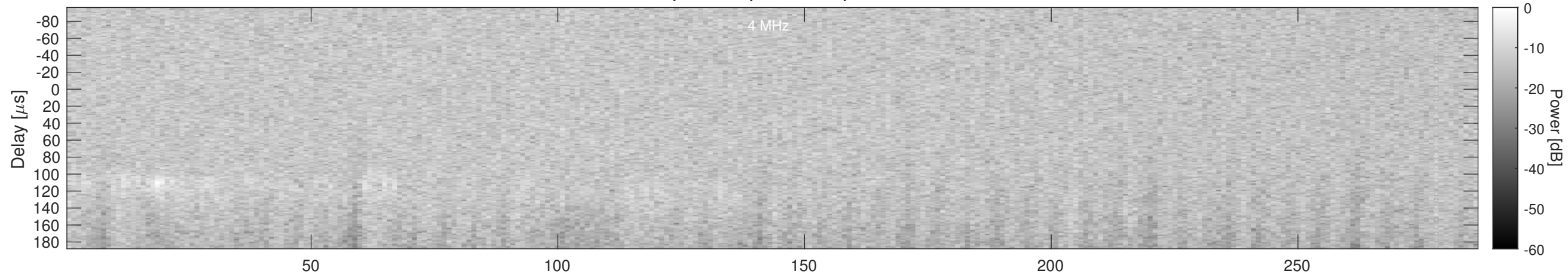
Orbit 4359, Window, Channel 2, Chapman
