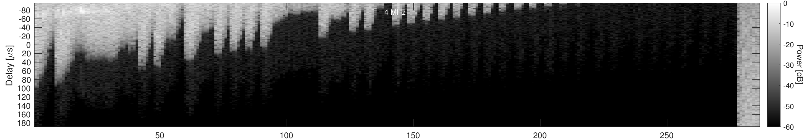
Orbit 4359, Window, Channel 2, Optimized
