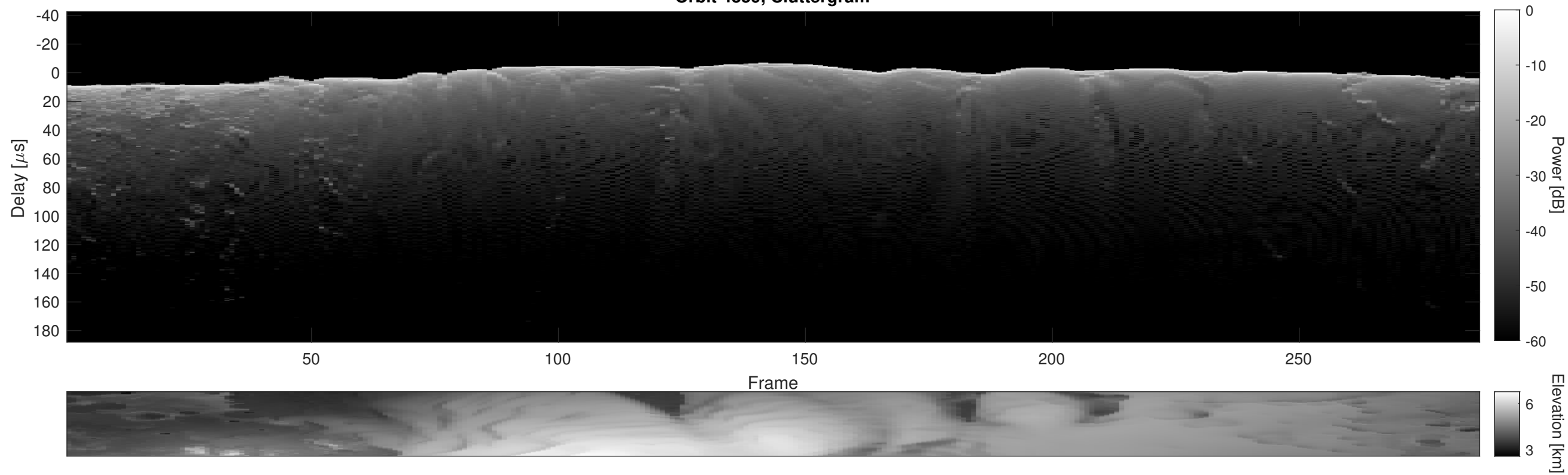
Orbit 4359, Cluttergram
