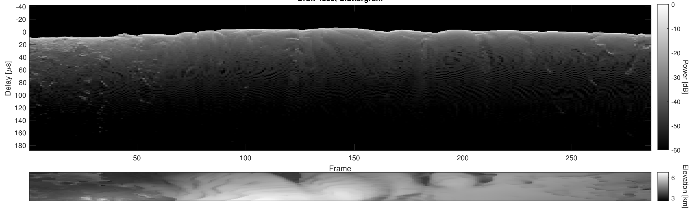
Orbit 4359, Cluttergram
