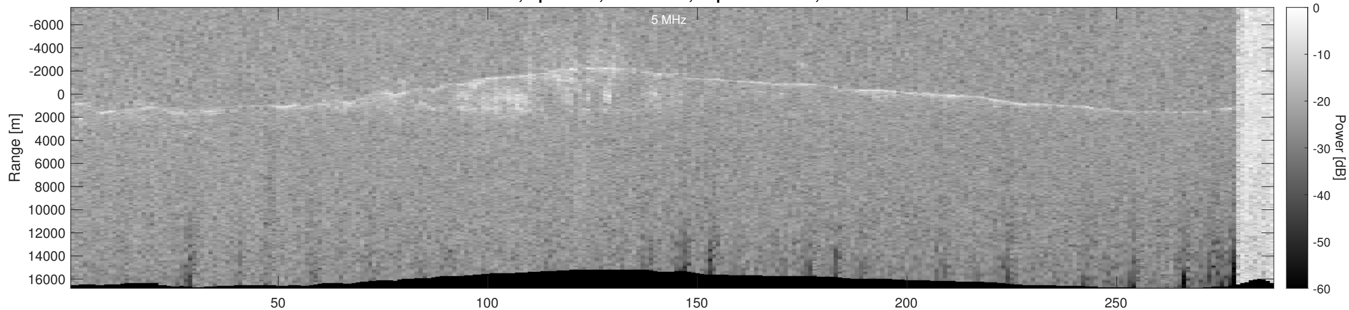
Orbit 4360, Optimized, No Window, Depth-Corrected, Channel 2
