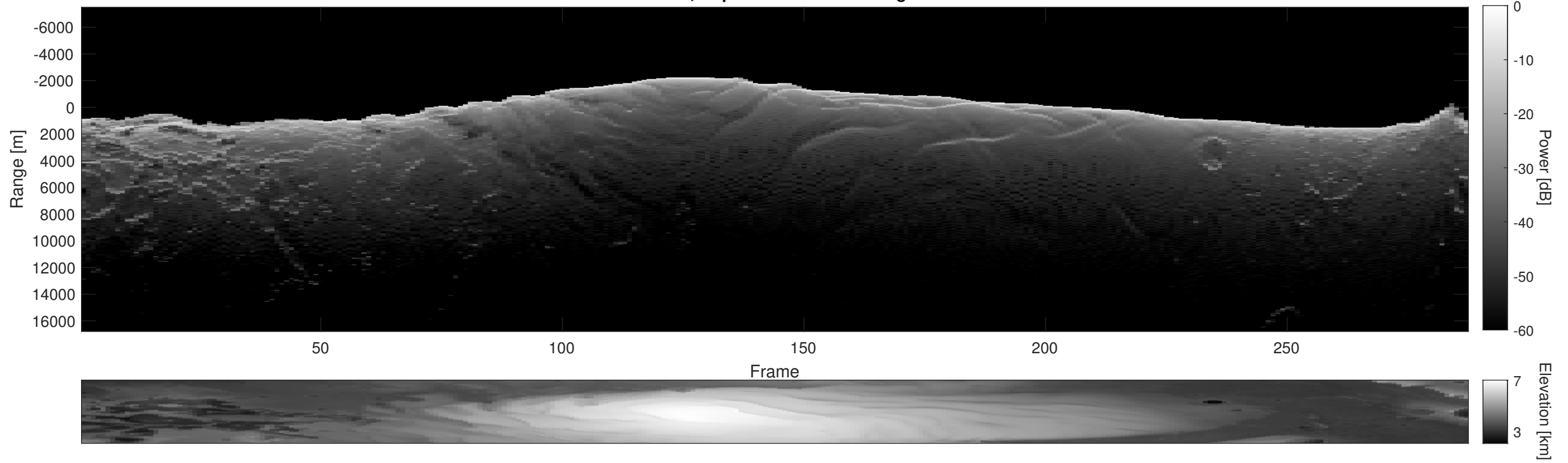
Orbit 4360, Depth-Corrected Cluttergram
