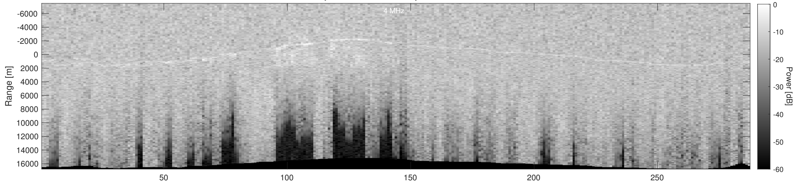
Orbit 4360, Depth-Corrected Cluttergram
