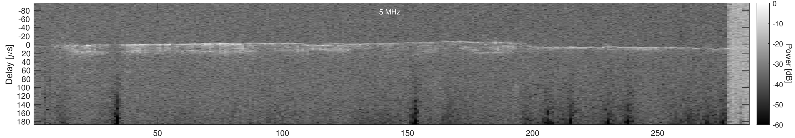
Orbit 4361, Cluttergram
