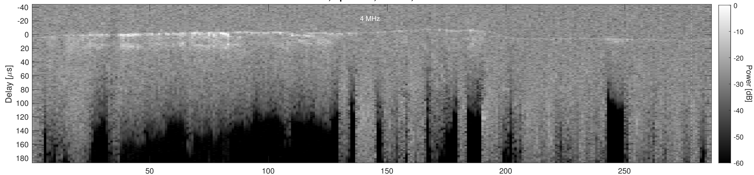
Orbit 4361, Cluttergram
