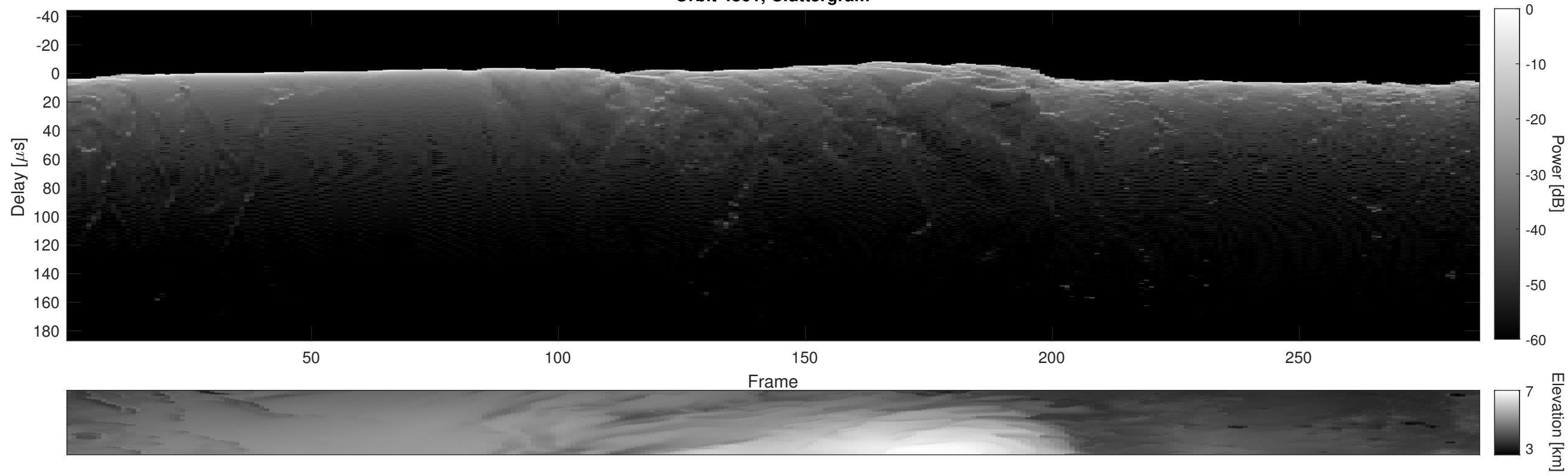
Orbit 4361, Cluttergram
