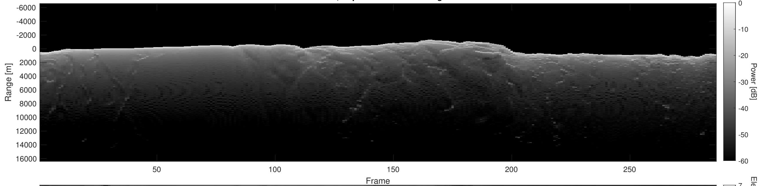
Orbit 4361, Depth-Corrected Cluttergram
