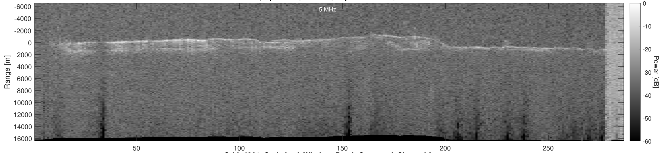
Orbit 4361, Optimized, Window, Depth-Corrected, Channel 2
