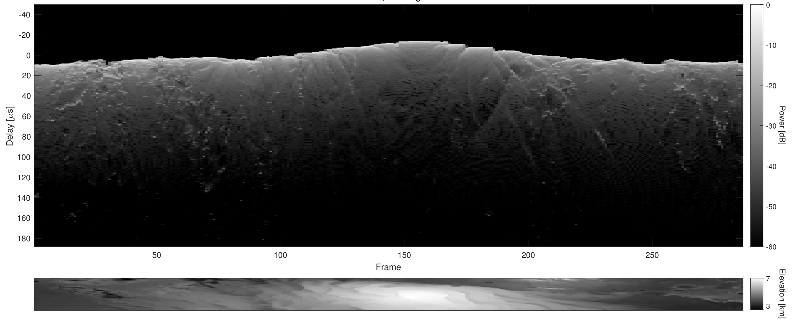
Orbit 4364, Cluttergram
