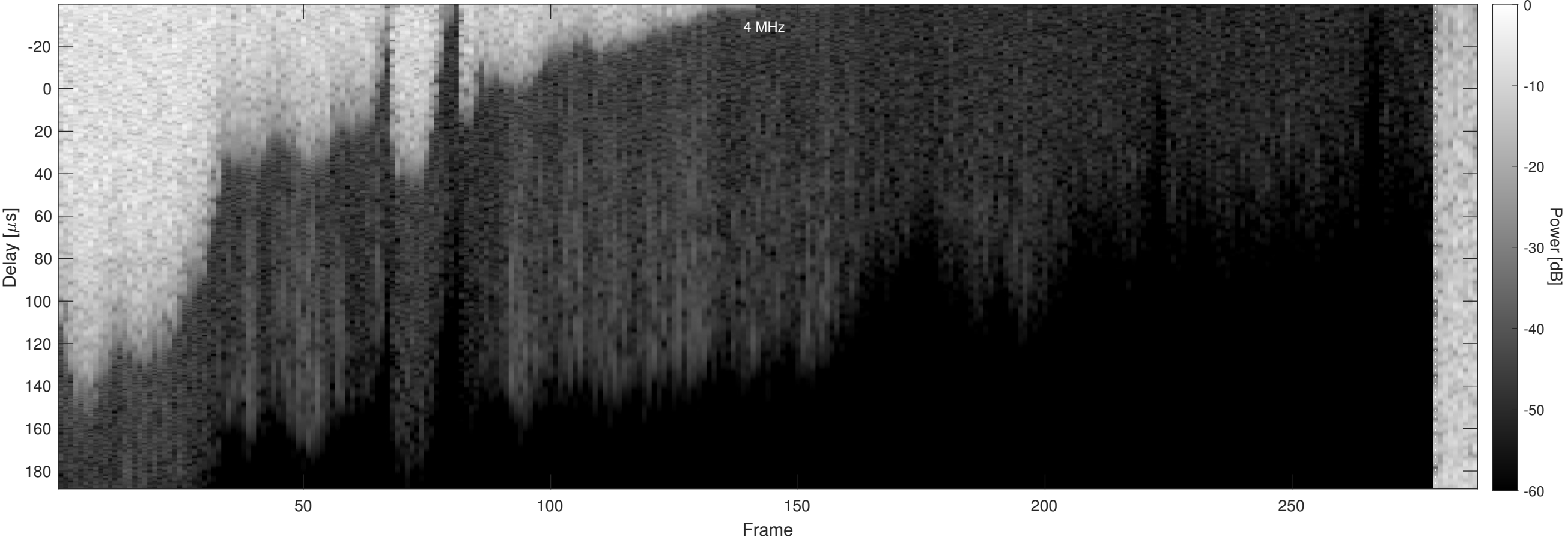
Orbit 4365, Chapman, Window, Channel 2
