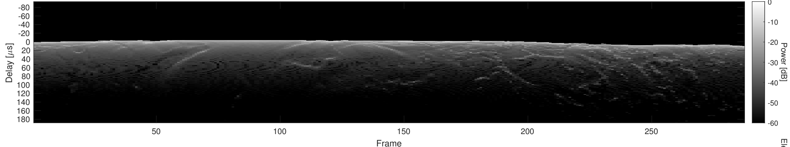
Orbit 4365, Cluttergram
