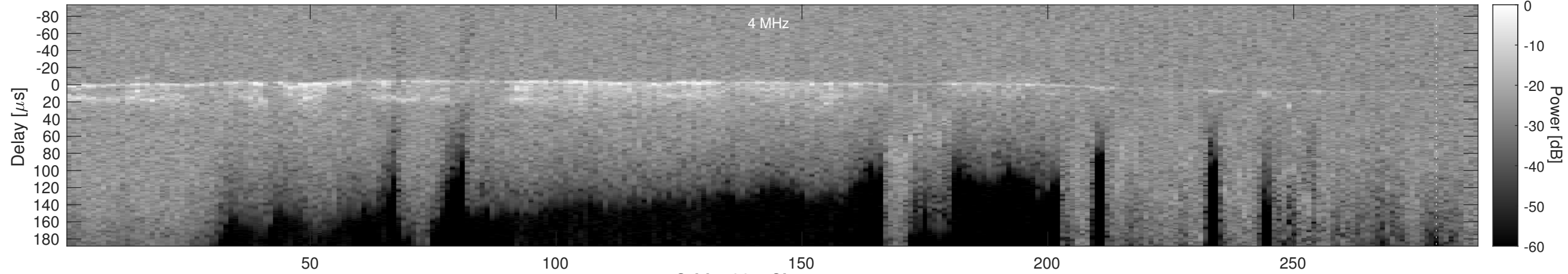
Orbit 4365, Cluttergram
