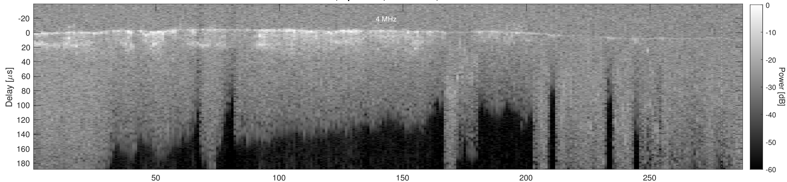
Orbit 4365, Cluttergram
