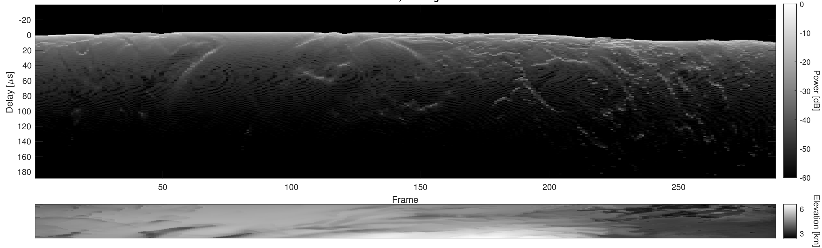
Orbit 4365, Cluttergram
