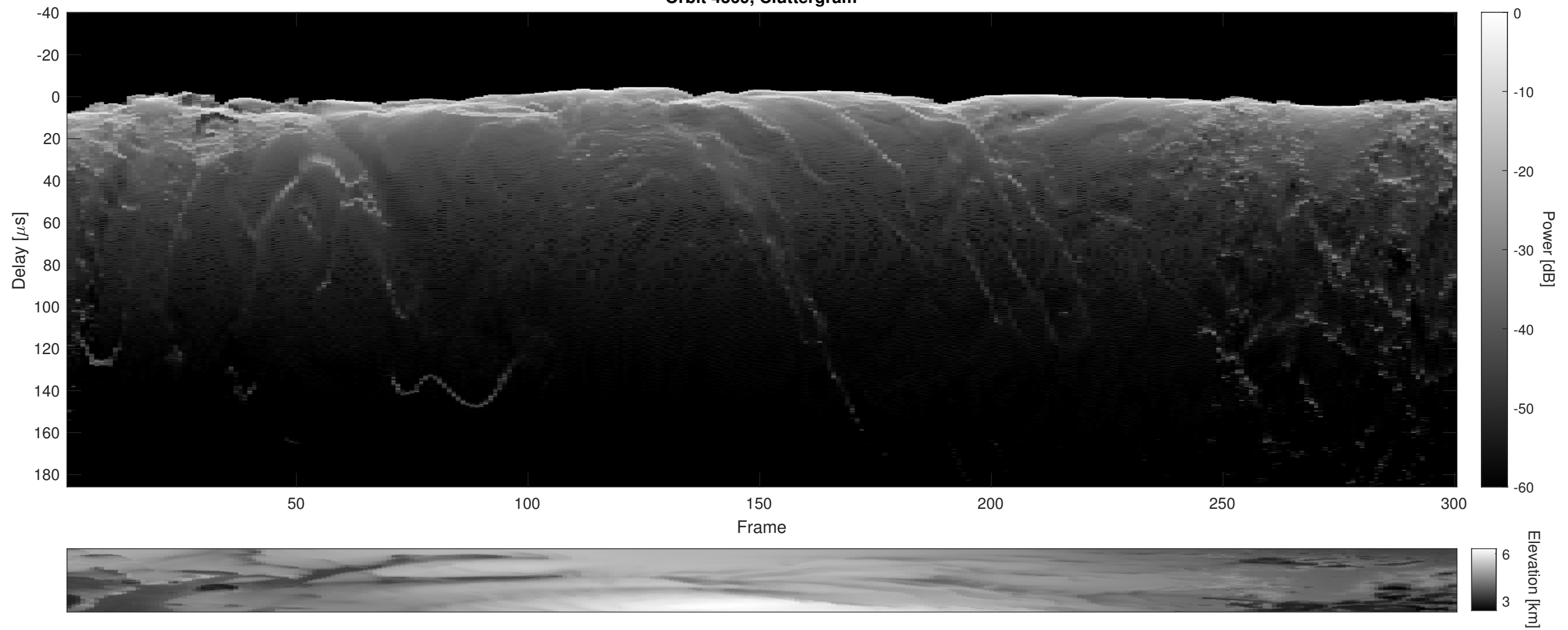
Orbit 4369, Cluttergram
