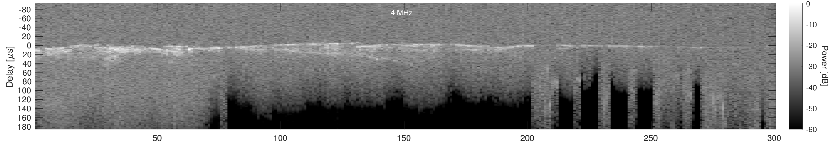
Orbit 4369, Cluttergram
