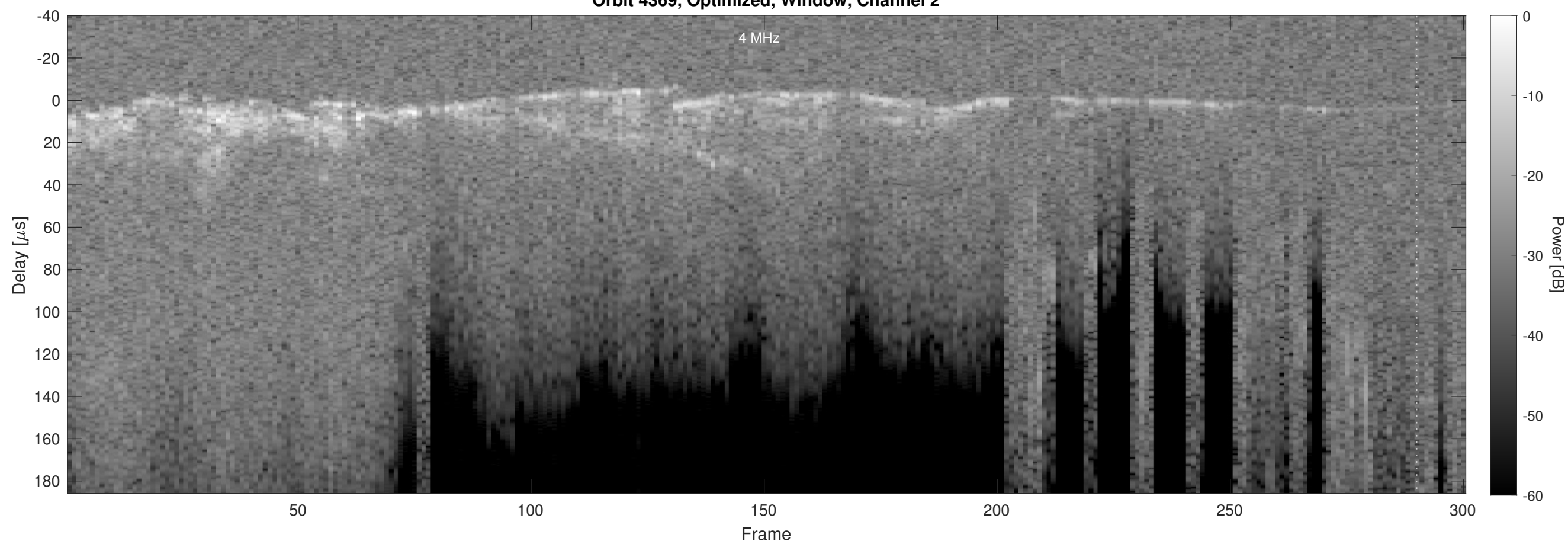
Orbit 4369, Optimized, Window, Channel 2
