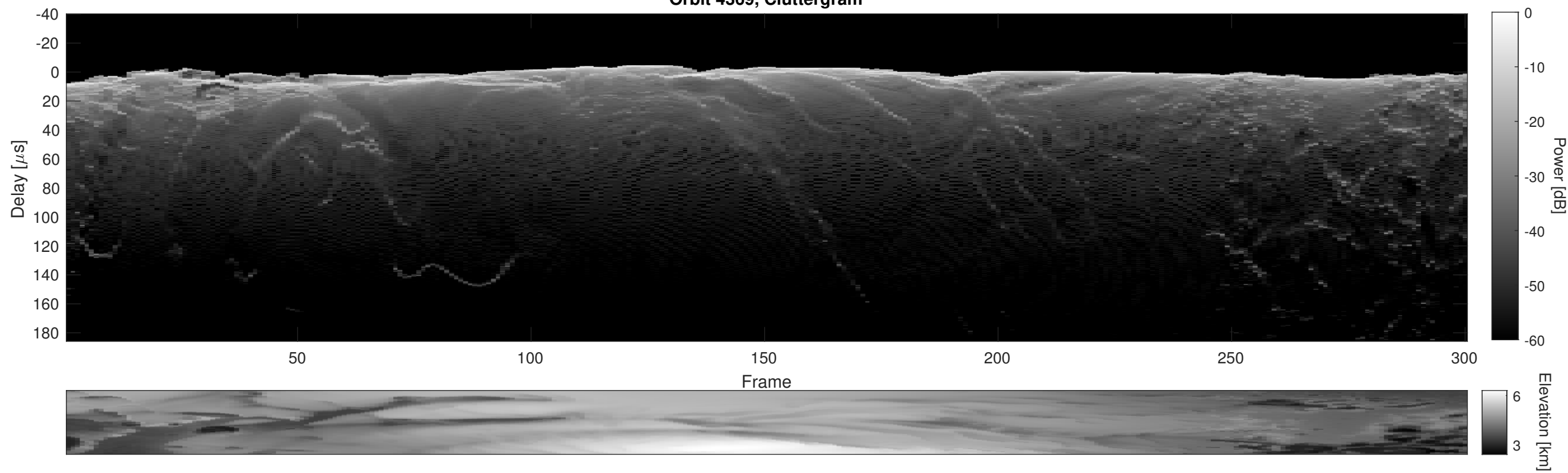
Orbit 4369, Cluttergram
