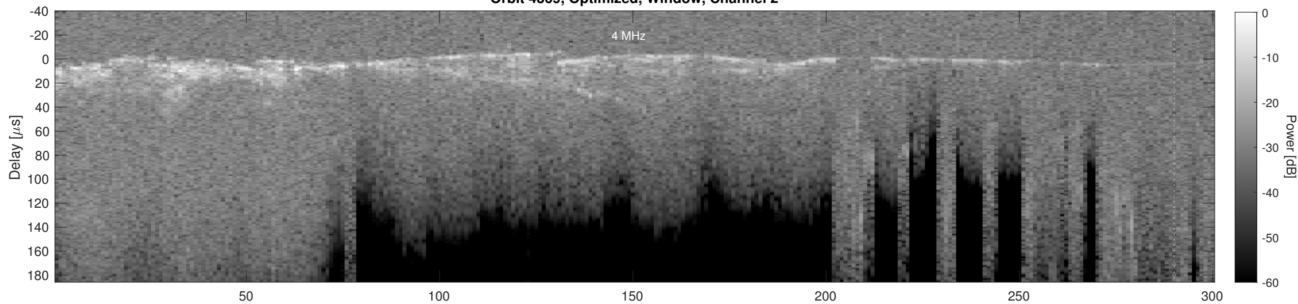
Orbit 4369, Cluttergram
