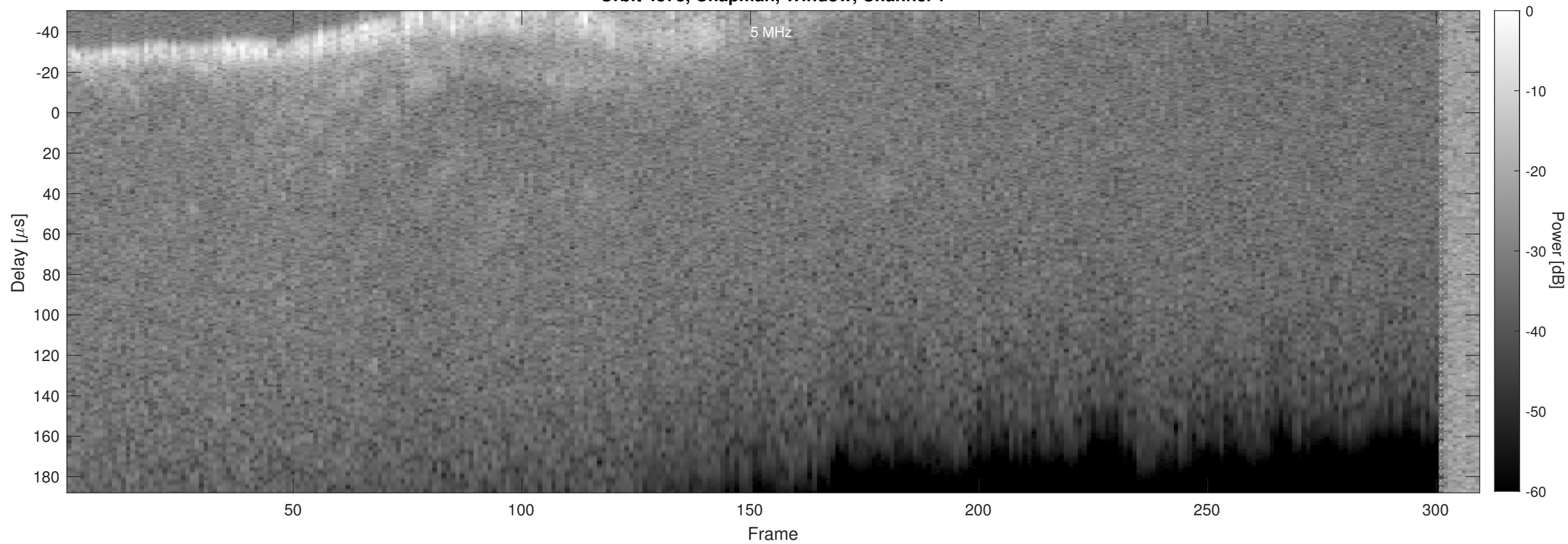
Orbit 4378, Chapman, Window, Channel 2
