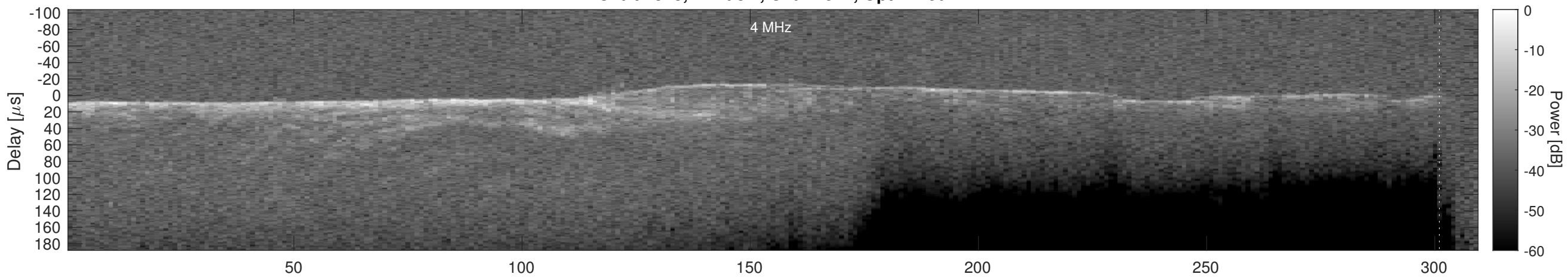
Orbit 4378, Cluttergram
