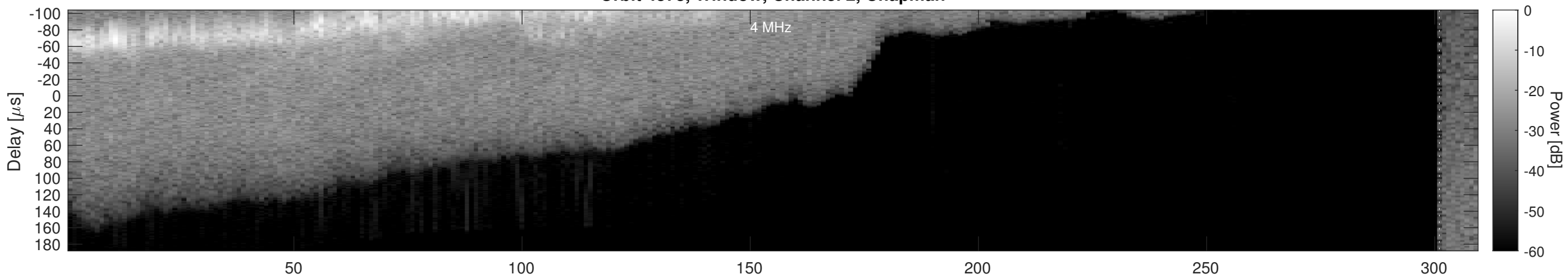
Orbit 4378, Window, Channel 2, Optimized
