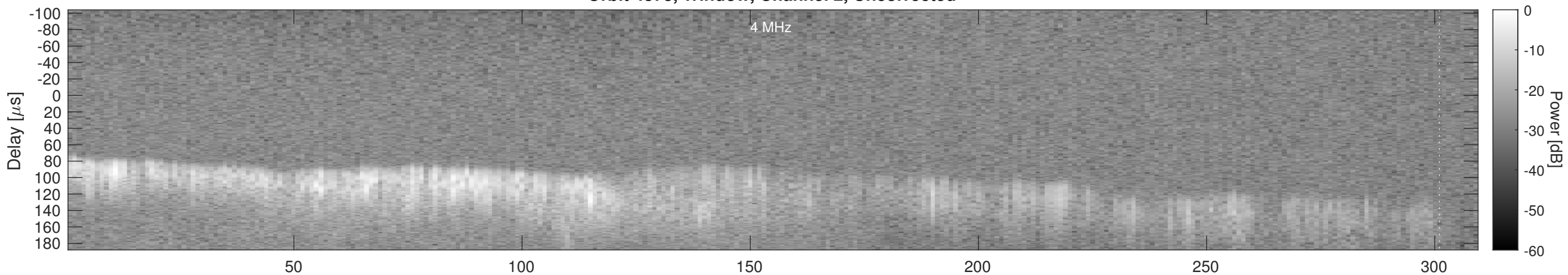
Orbit 4378, Window, Channel 2, Chapman
