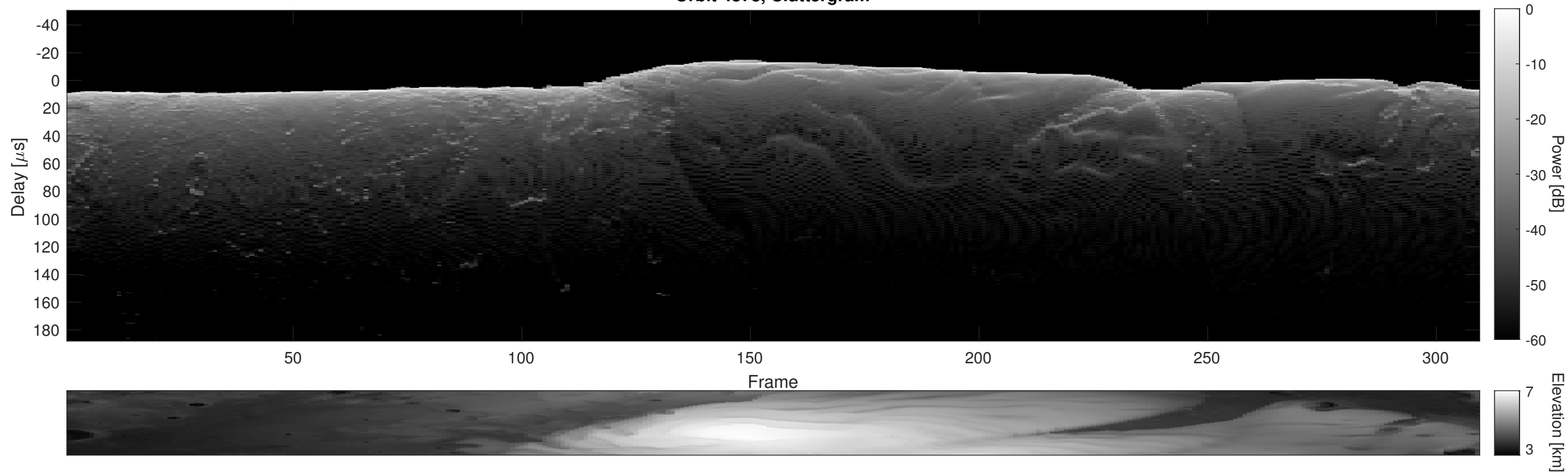
Orbit 4378, Cluttergram
