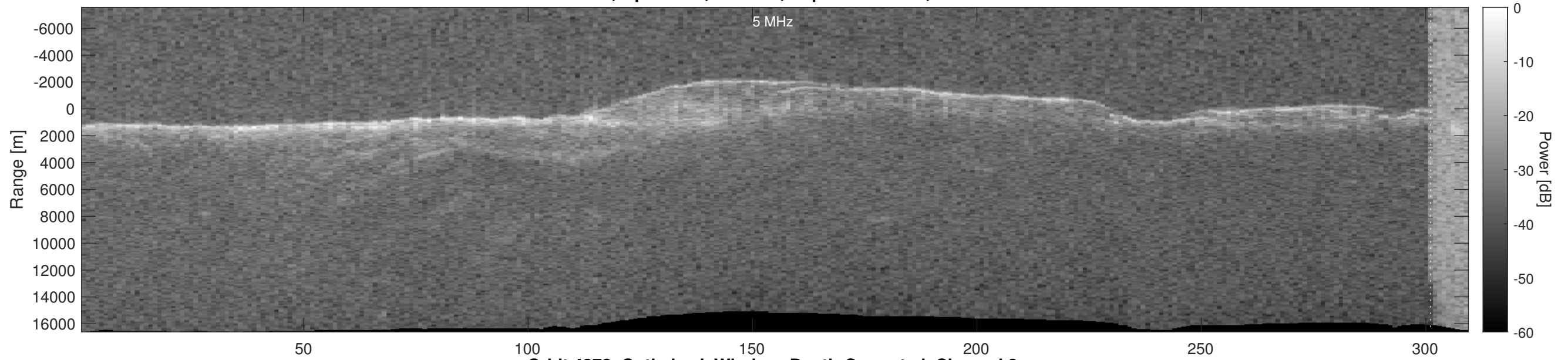
Orbit 4378, Optimized, Window, Depth-Corrected, Channel 2
