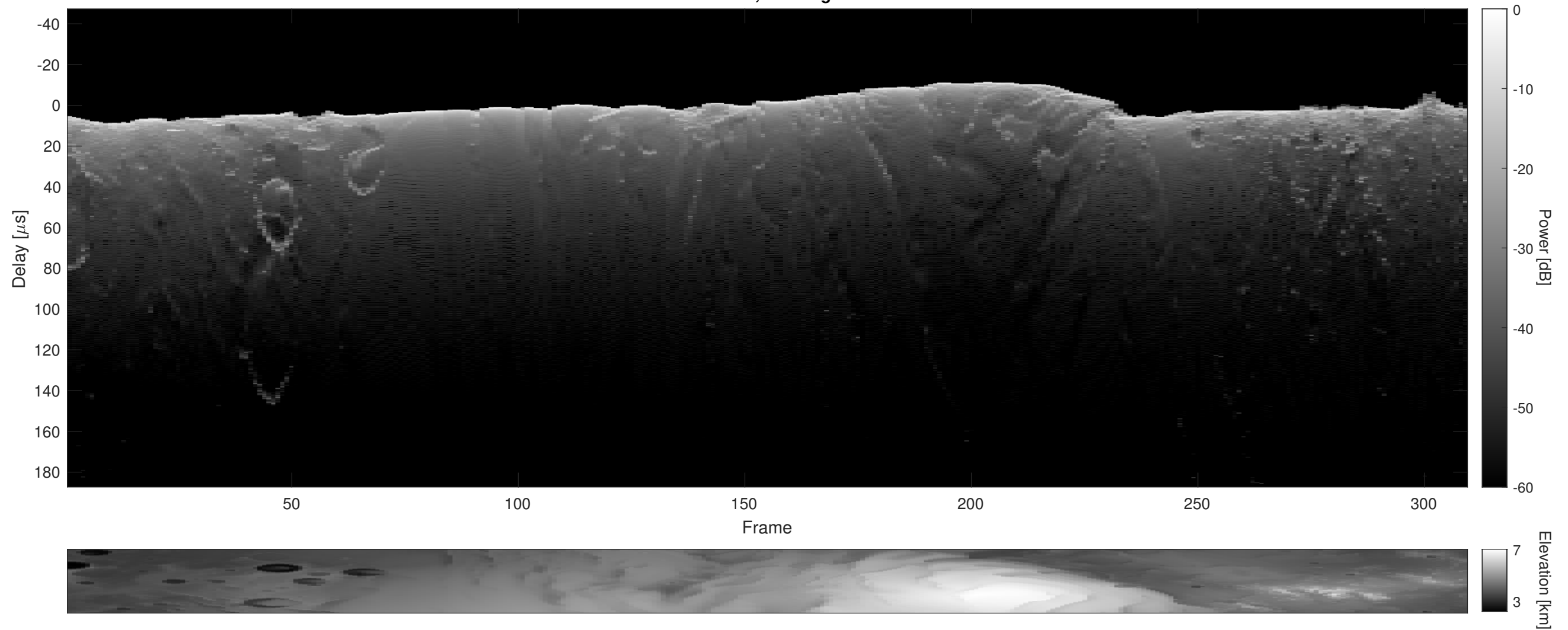
Orbit 4379, Cluttergram
