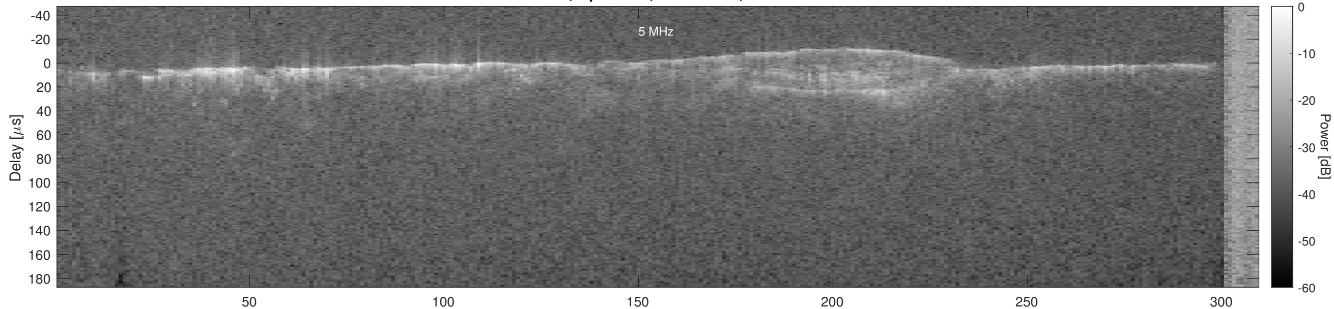
Orbit 4379, Optimized, No Window, Channel 2
