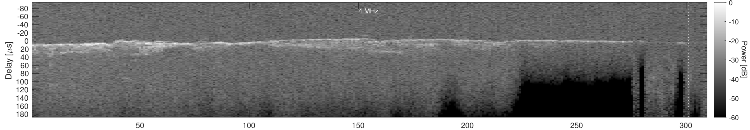
Orbit 4380, Cluttergram
