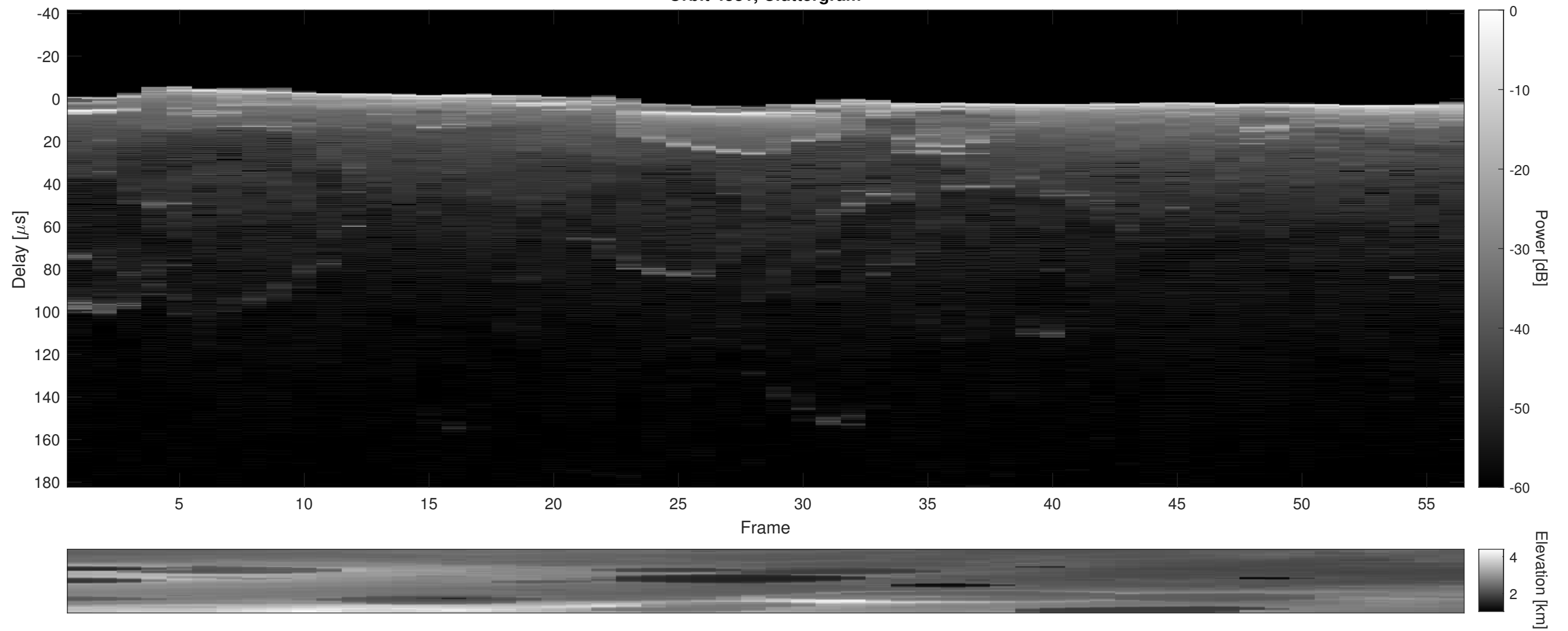
Orbit 4381, Cluttergram
