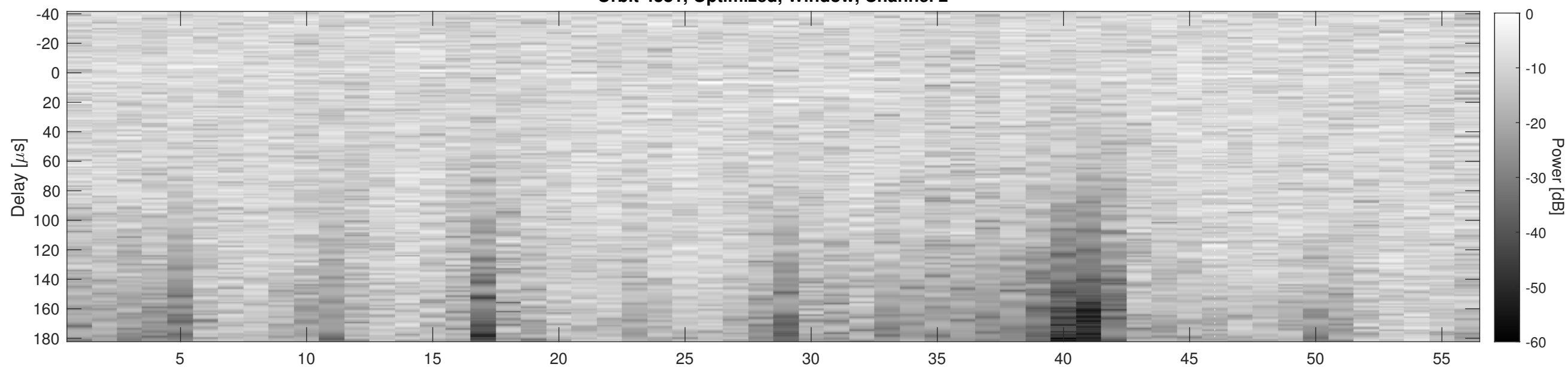
Orbit 4381, Cluttergram
