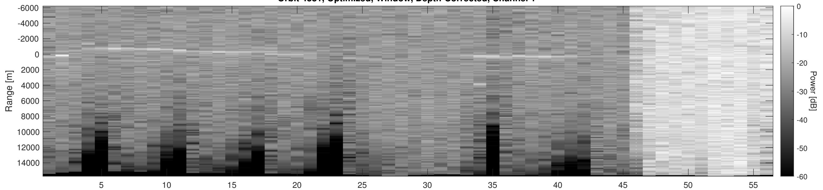
Orbit 4381, Optimized, Window, Depth-Corrected, Channel 2
