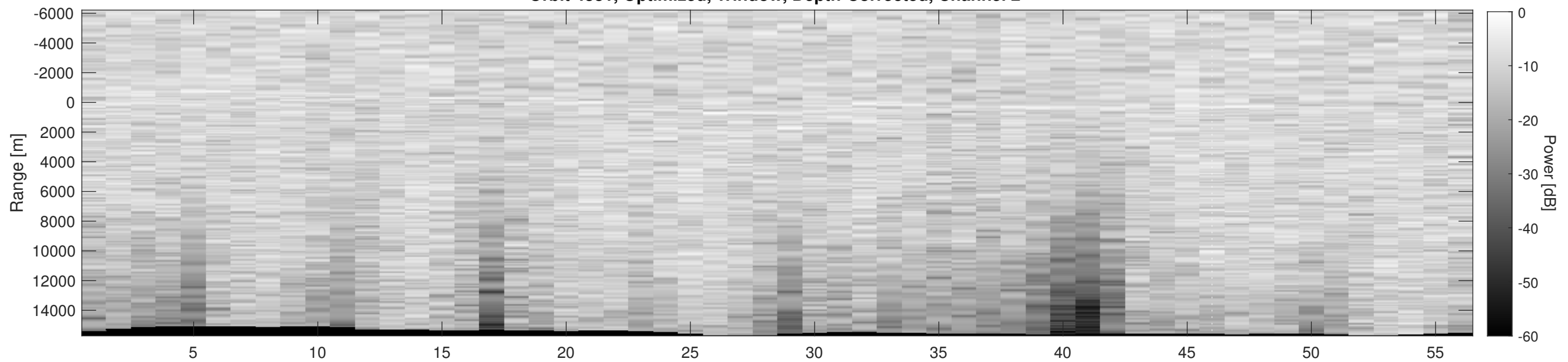
Orbit 4381, Depth-Corrected Cluttergram
