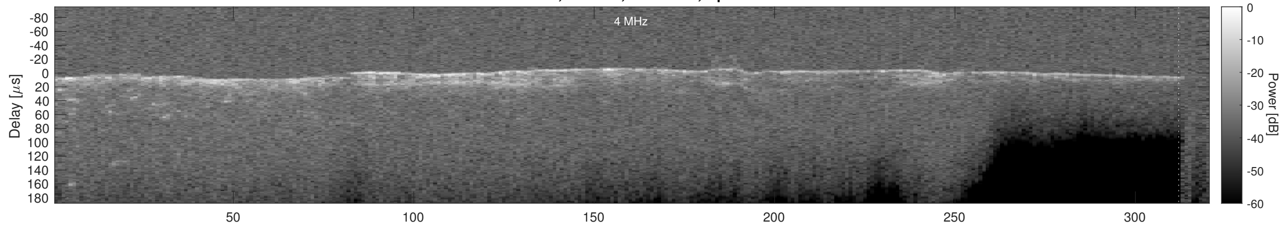
Orbit 4384, Cluttergram
