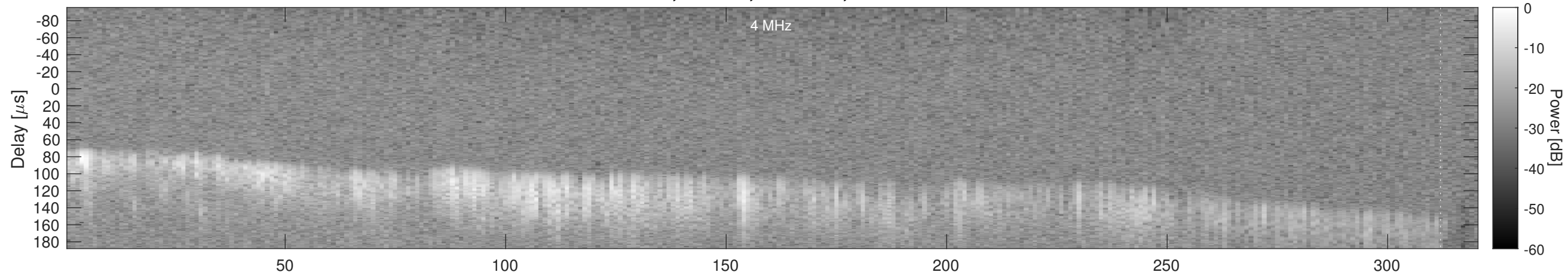
Orbit 4384, Window, Channel 2, Chapman
