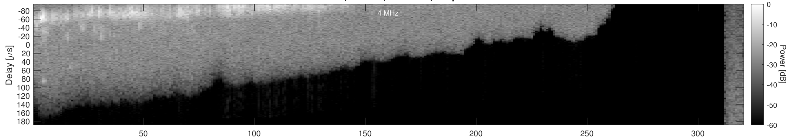
Orbit 4384, Window, Channel 2, Optimized
