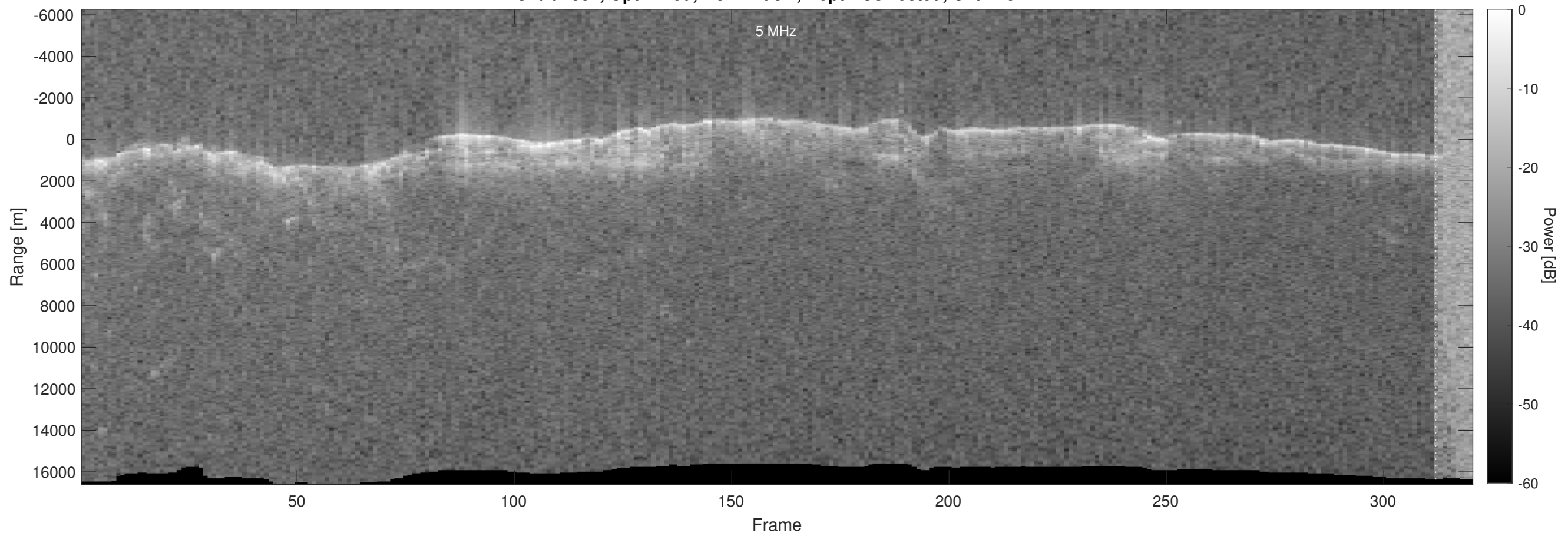
Orbit 4384, Optimized, No Window, Depth-Corrected, Channel 2
