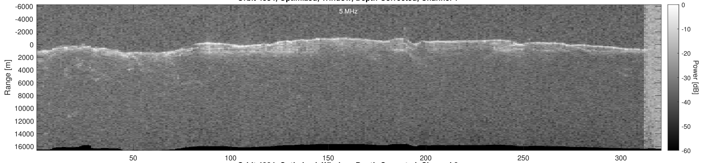
Orbit 4384, Optimized, Window, Depth-Corrected, Channel 2
