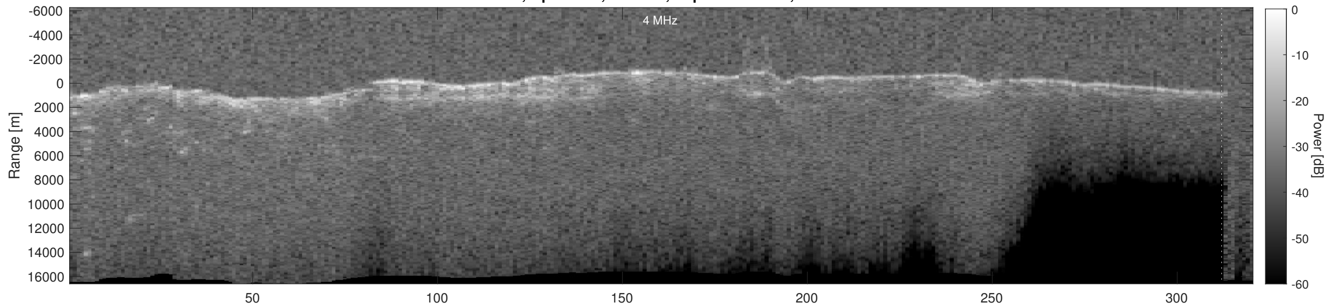
Orbit 4384, Depth-Corrected Cluttergram
