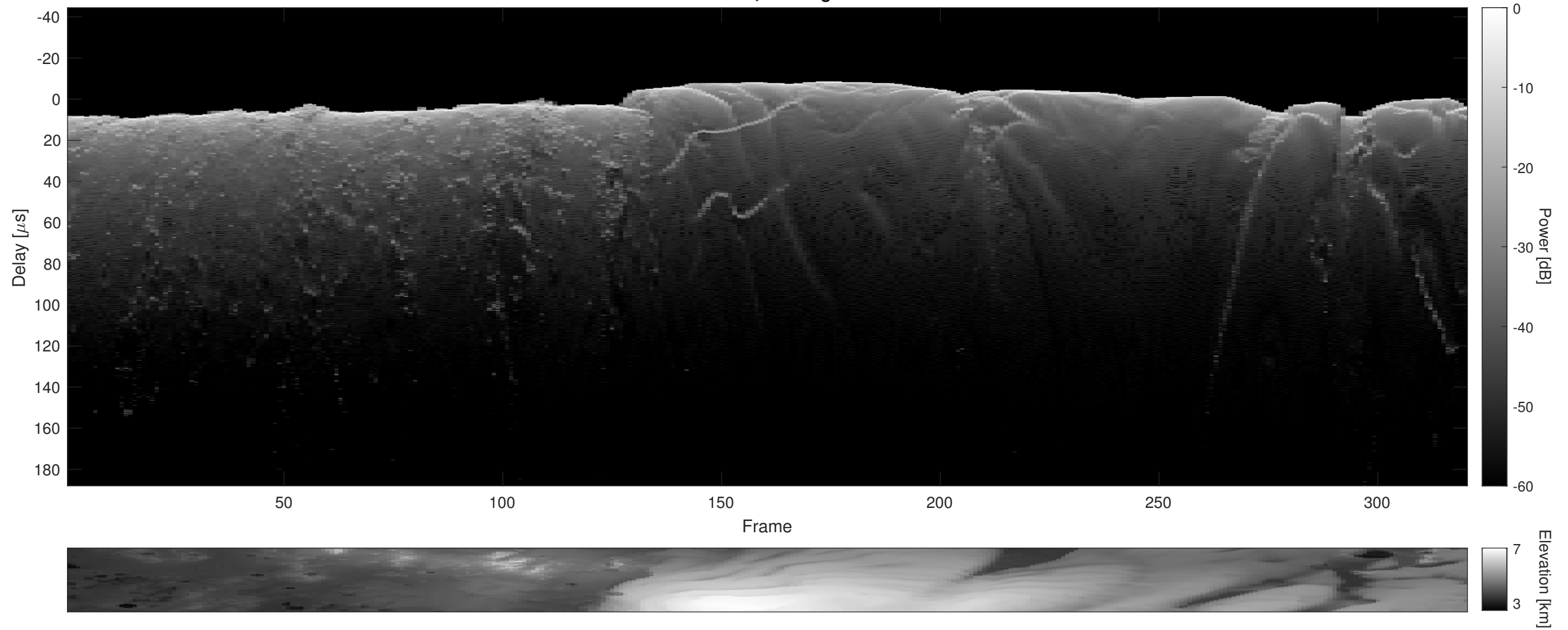
Orbit 4385, Cluttergram
