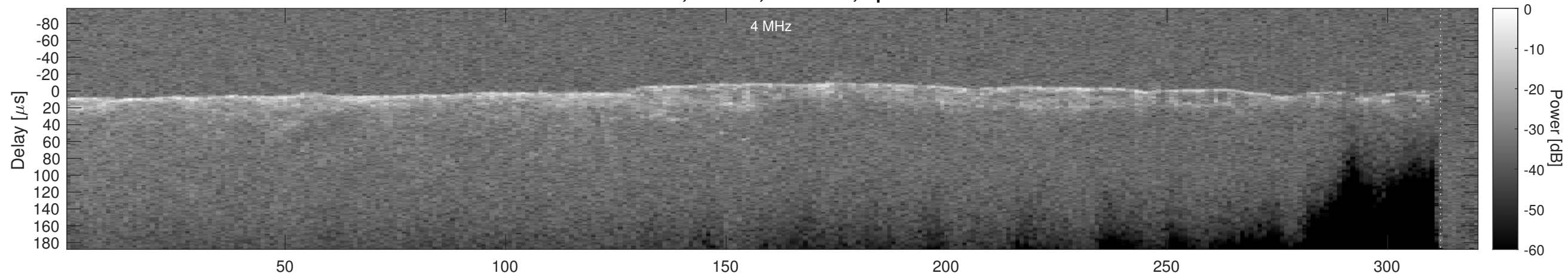
Orbit 4385, Cluttergram
