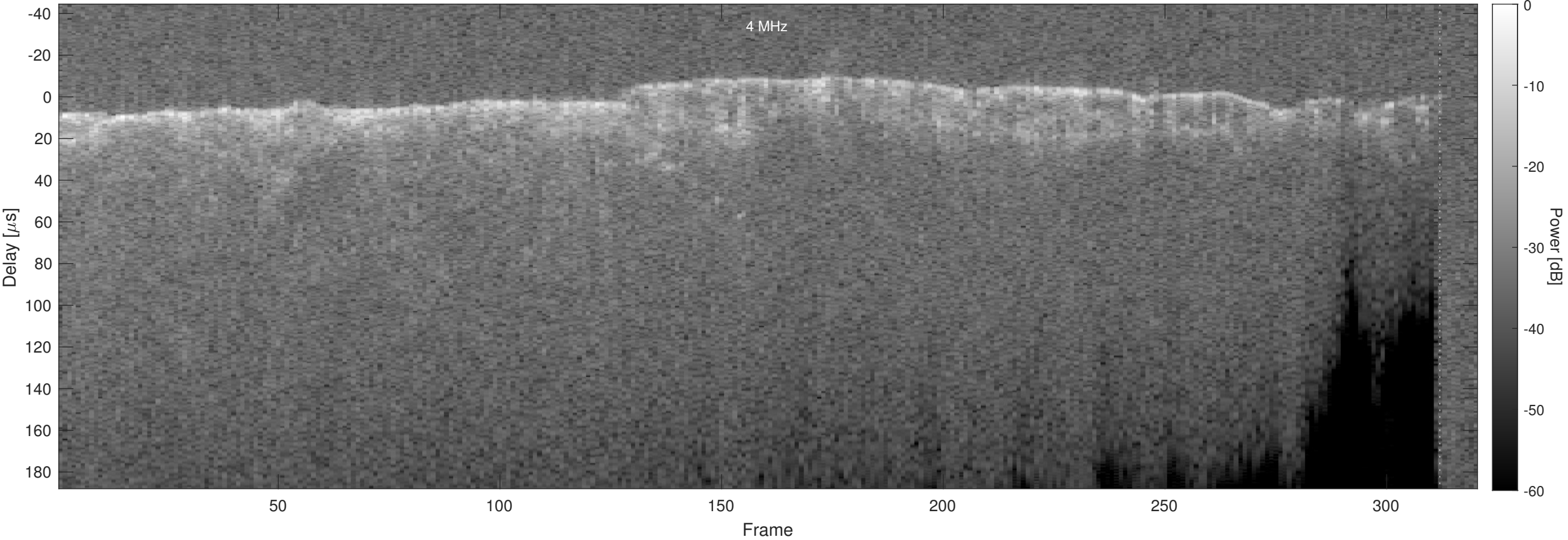
Orbit 4385, Optimized, No Window, Channel 2
