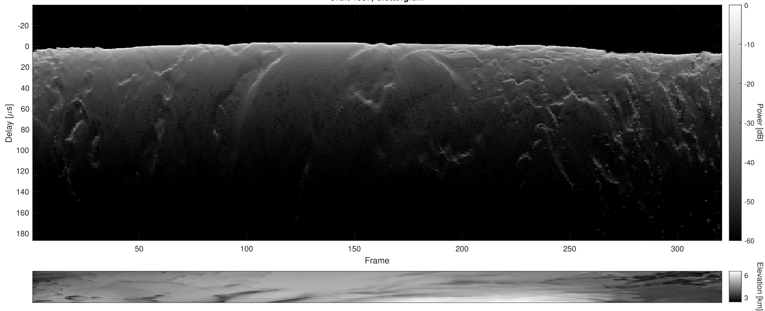
Orbit 4387, Cluttergram
